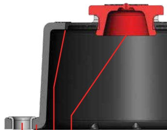
Vent Permanent Bond Sealing Ring Stainless Steel Insert
